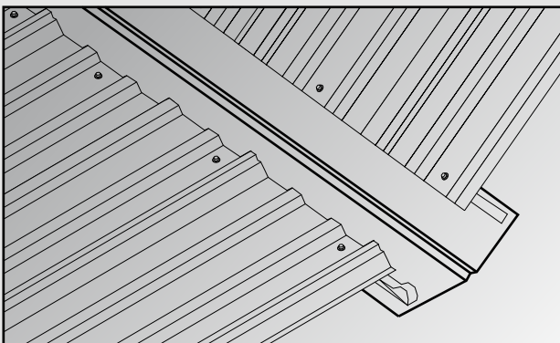
Valley Trim
