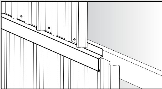
Wainscoat Trim
