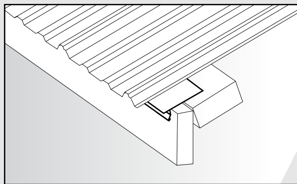
Residential Eave
